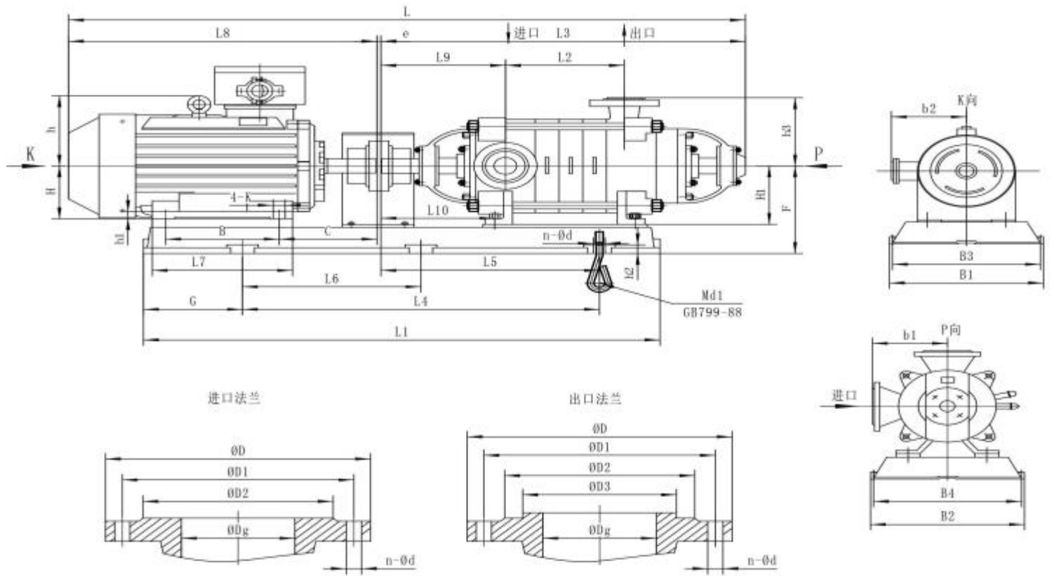
D型多级离心泵外形安装图（电机、泵共同底座） Installation diagram of D-type multi-stage centrifugal pump (motor and pump share the same base)
