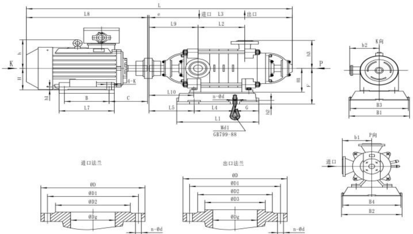
D型多级离心泵外形安装图（单泵底座） Installation diagram of D type multi-stage centrifugal pump (single pump base)
